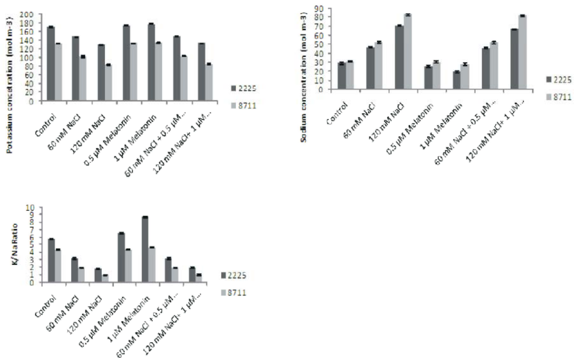
Fig. 3: Effect of melatonin on ionic attributes of two maize hybrids under salt stress. The bars in the graph show average values of five replicates and the error bars are the standard deviations
